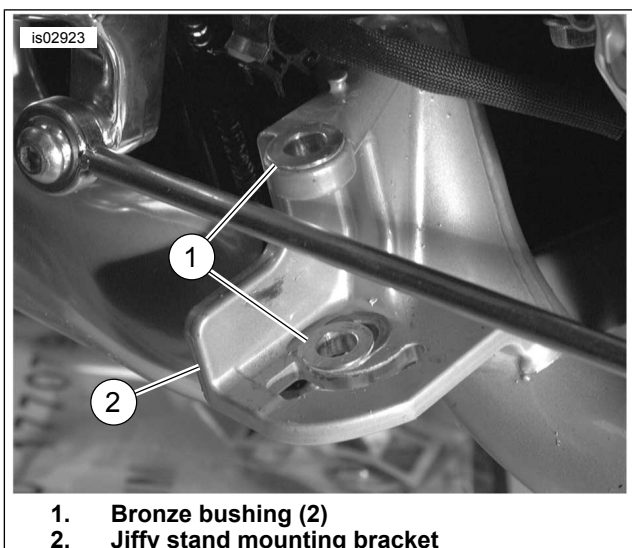
Figure 2. Jiffy Stand Mounting Bracket
