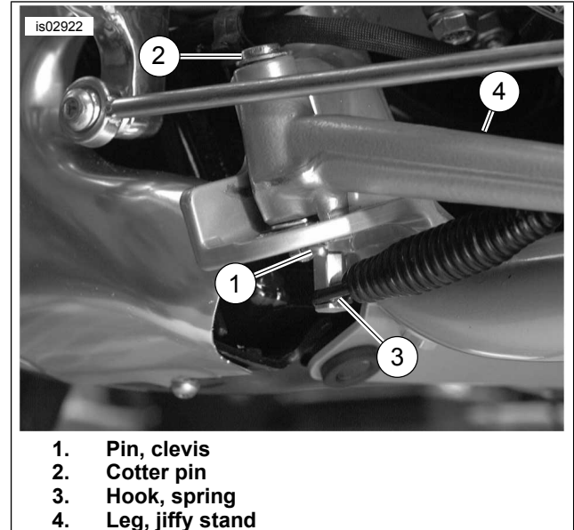
Figure 1. Jiffy Stand Components
