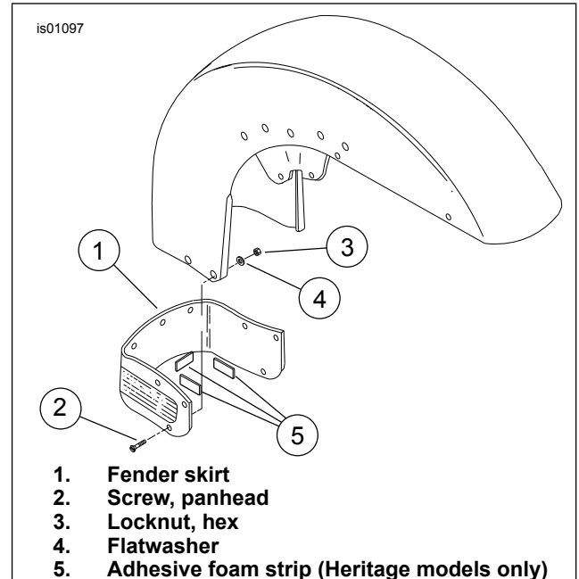
Figure 1. Front Fender Skirt and Assembling Hardware
