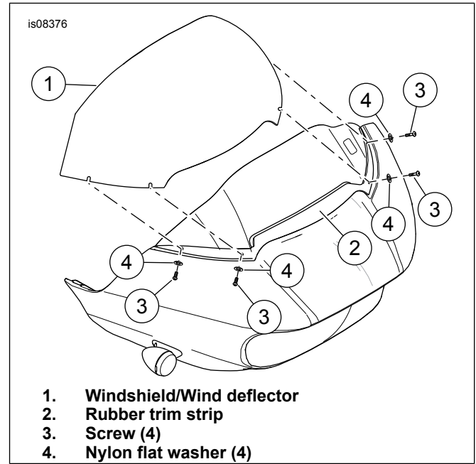
Figure 1. Windshield/Wind Deflector Installation
