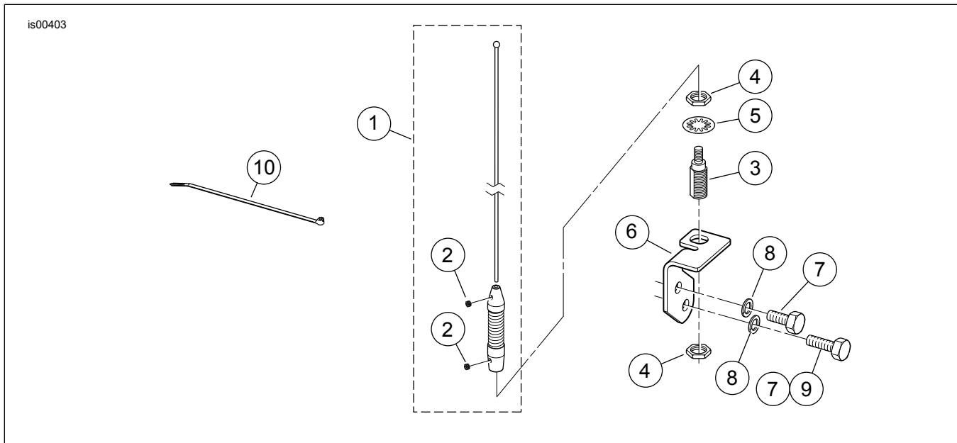
Figure 2. Service Parts, AM/ FM Frame Mount Antenna
