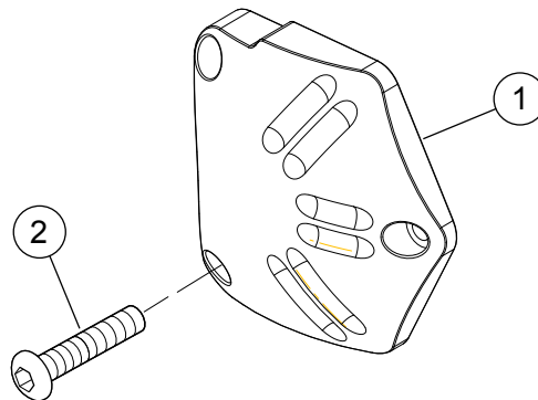
Figure 1. Service Parts: Solenoid Cover
