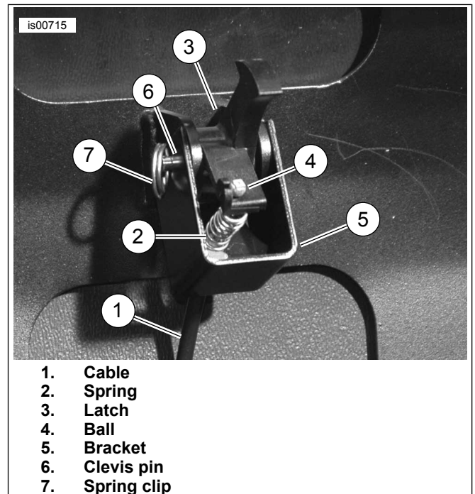
Figure 7. Install Latch and Spring Kit
