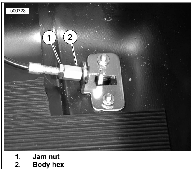
Figure 8. Adjust Cable Assembly
