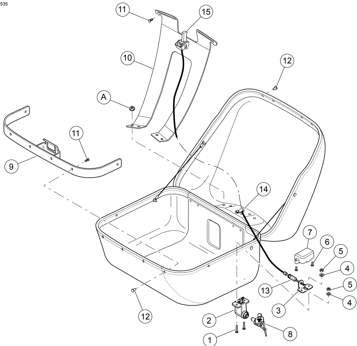
Figure 9. Service Parts: Leather Tour-Pak Lock
