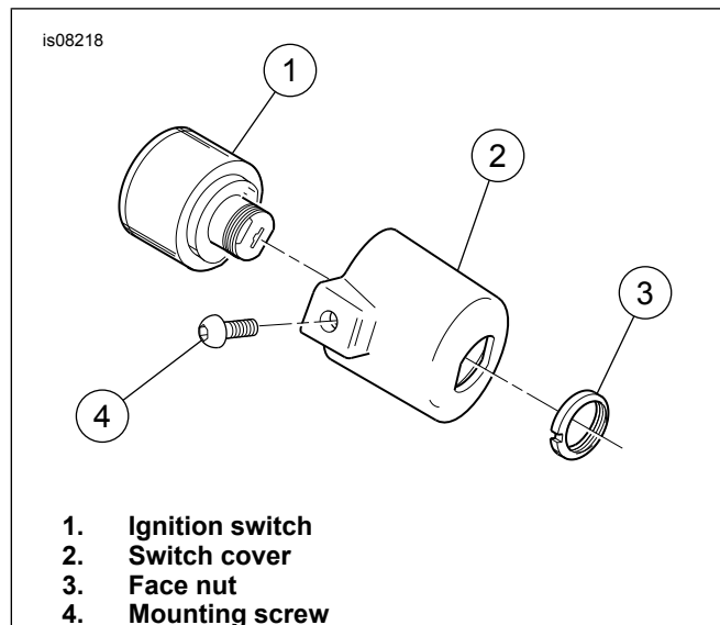
Figure 1. Ignition Switch Cover Installation
