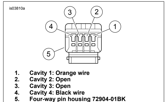
Figure 3. Four-Way Pin Housing (Viewed From Wire End)
