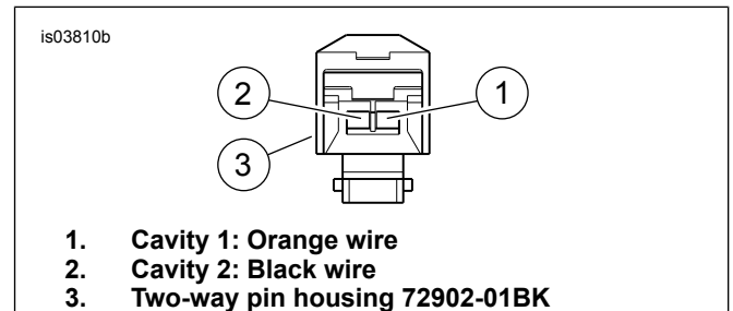
Figure 4. Two-Way Pin Housing (Viewed From Wire End)
