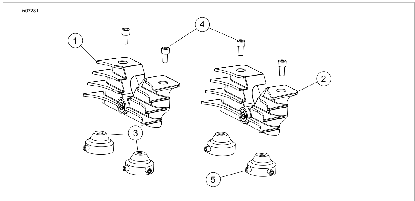
Figure 1. Service Parts: Finned Headbolt Cover Kit
