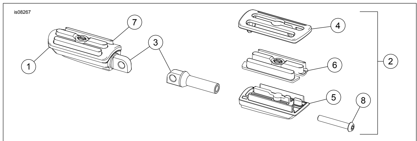
Figure 2. Service Parts
