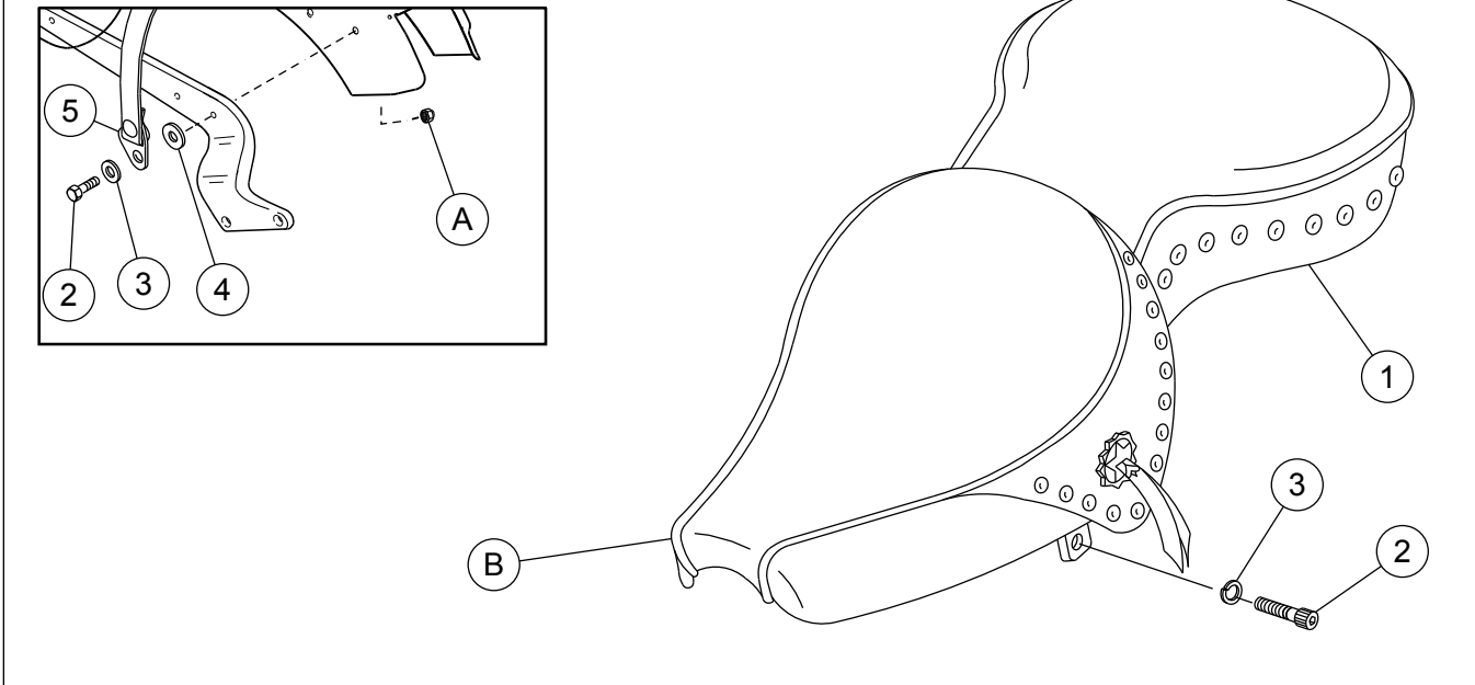
Figure 1. Service Parts: FLSTC Touring Pillion
