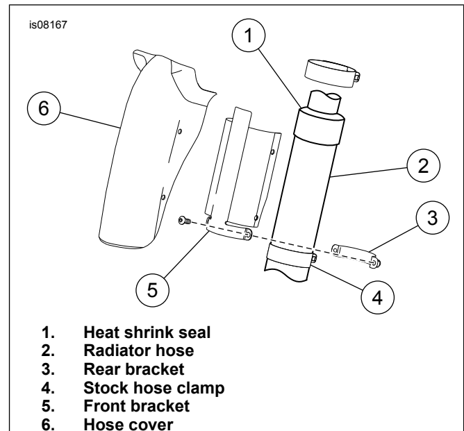
Figure 1. Hose Cover and Hose Components
