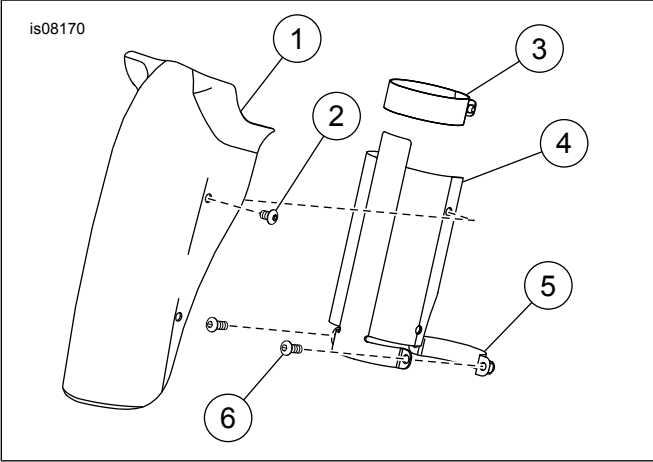
Figure 4. Service Parts
