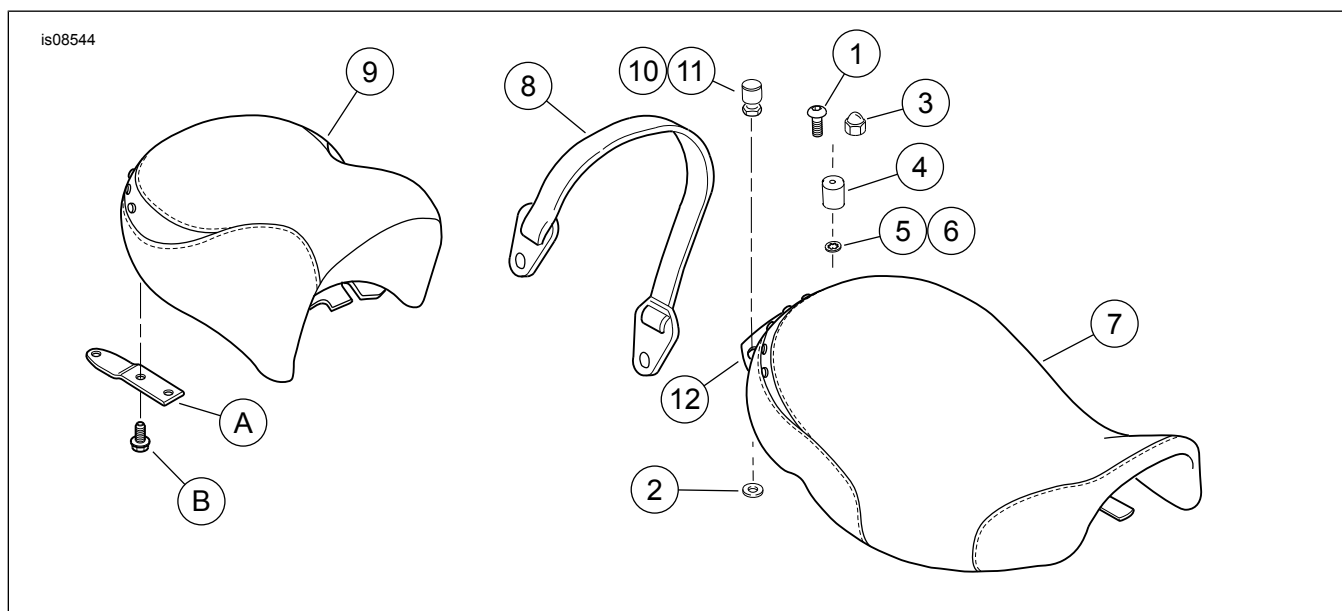
Figure 1. Service Parts: Road King Solo Bucket and Pillion
