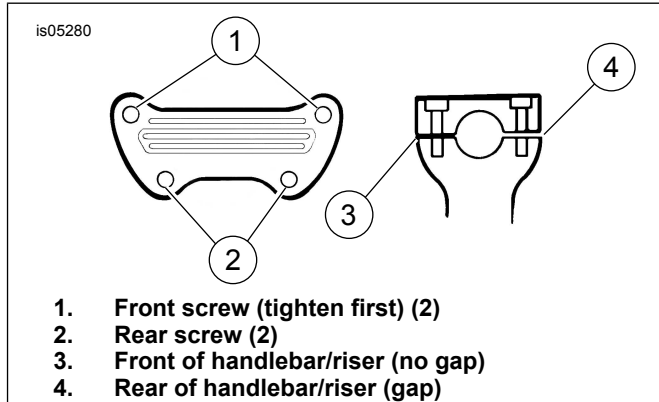
Figure 1. Handlebar Mounting
