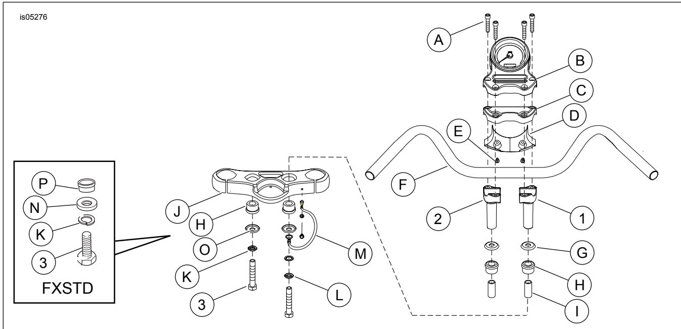
Figure 2. Service Parts: Tall Handlebar Riser
