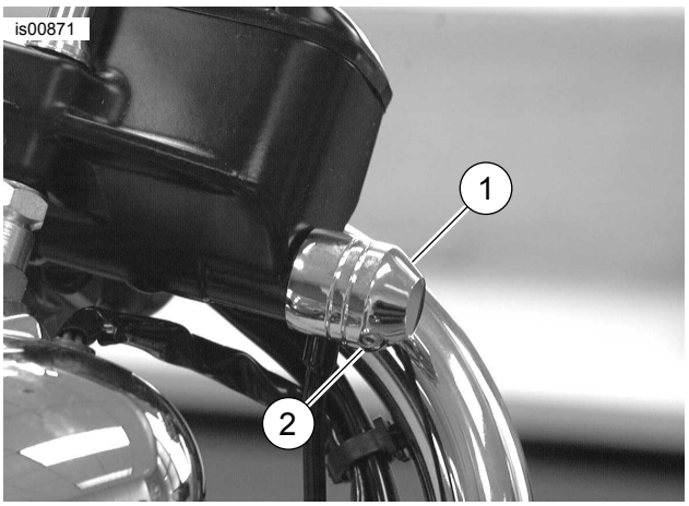
Figure 4. Set Screw Location on Banjo Bolt Cover
