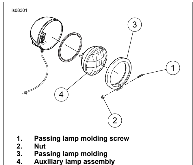
Figure 1. Auxiliary Lamp Components
