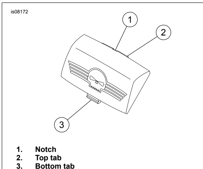
Figure 1. Fender-Tip Lens
