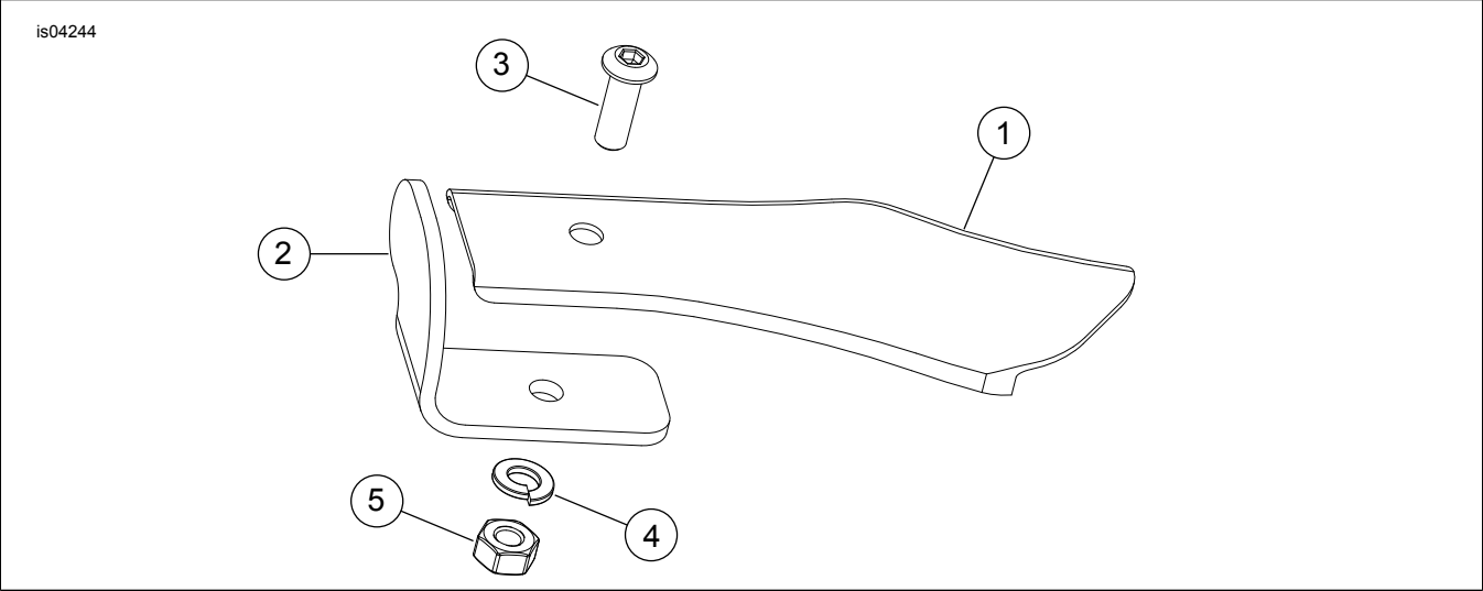
Figure 2. Service Parts: XL Jiffy Stand Extension Kit
