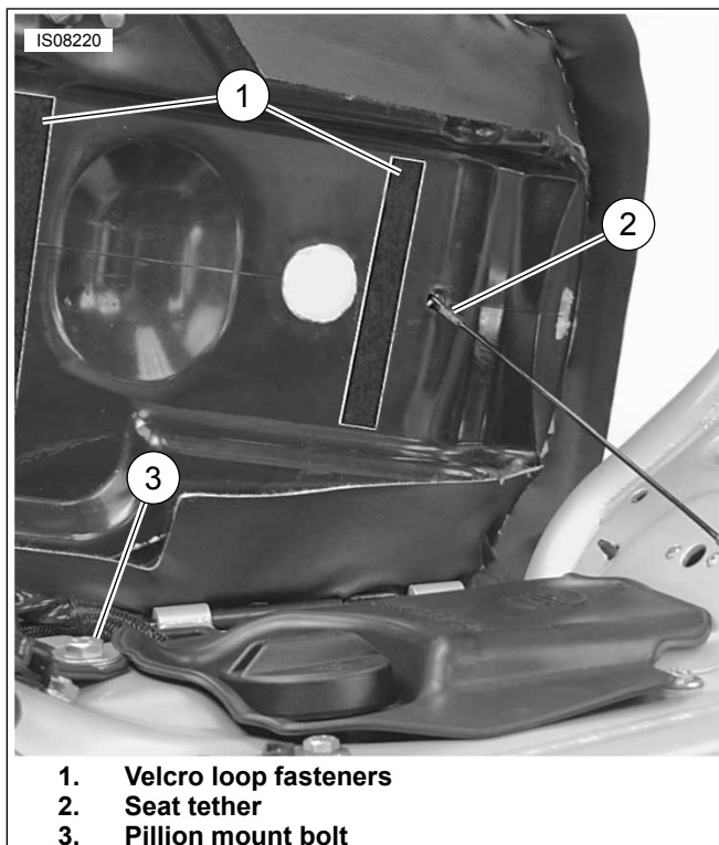
Figure 1. Positioning the Velcro Loop Fasteners
