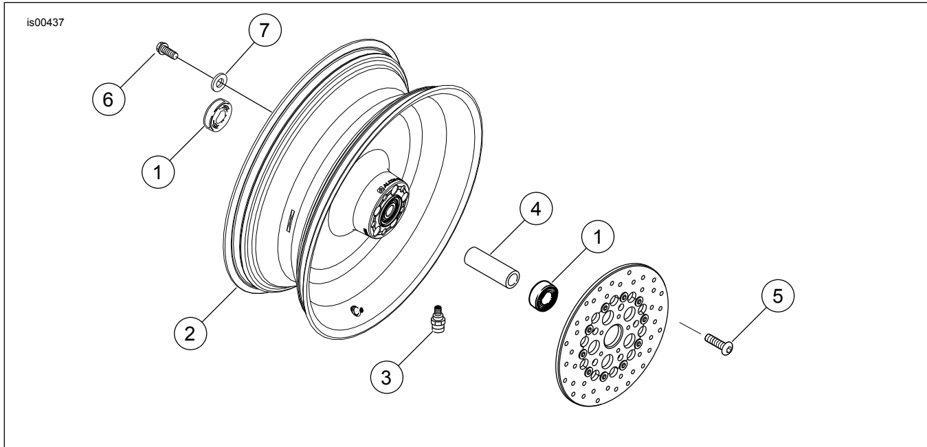
Figure 1. Service Parts: Chrome 17 Inch Rear Wheel Kits (solid dish wheel shown)
