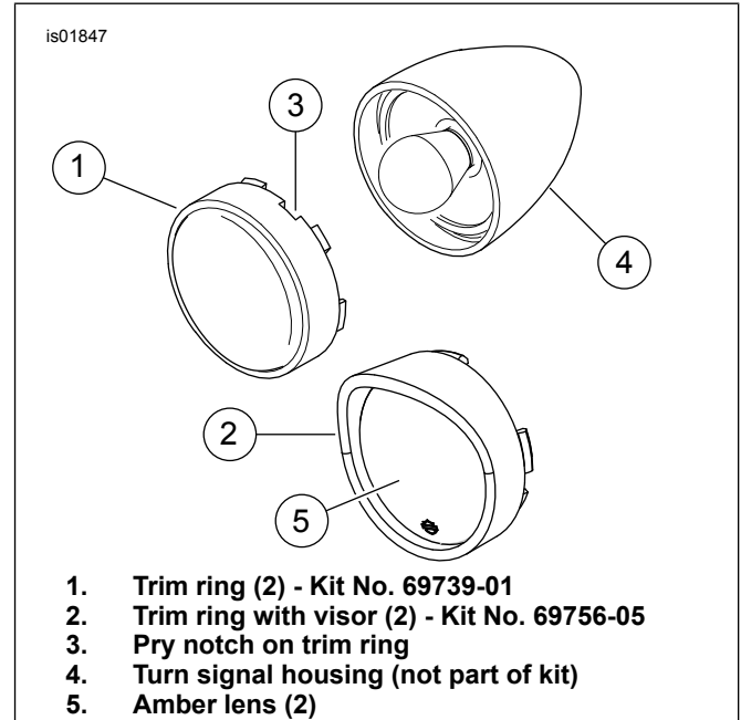
Figure 1. Bullet-Style Turn Signal Lens
