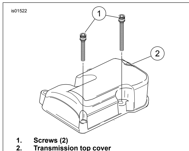
Figure 1. Transmission Top Cover Screws
