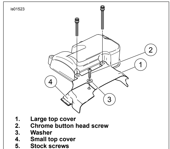
Figure 2. Cover Assembly
