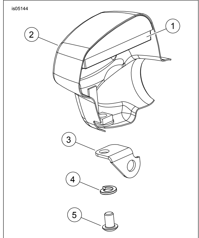
Figure 2. Service Parts: Master Cylinder Cover Kit
