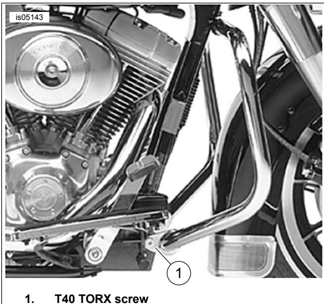
Figure 1. Lower Engine Guard TORX Screw
