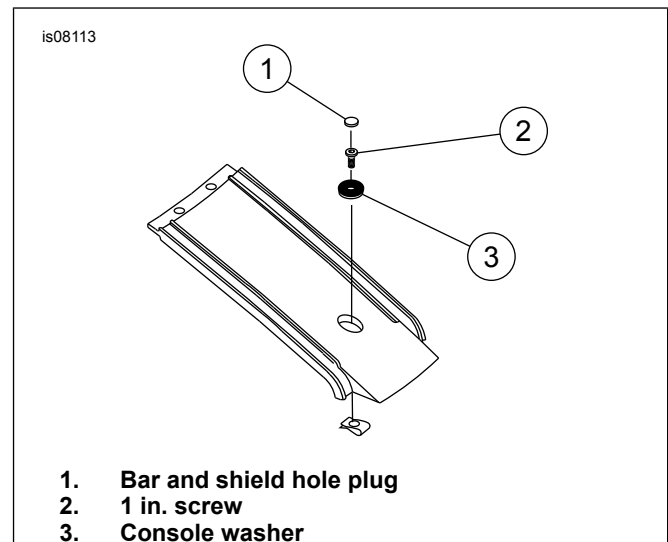
Figure 2. Installation on Softail Tank Panel
