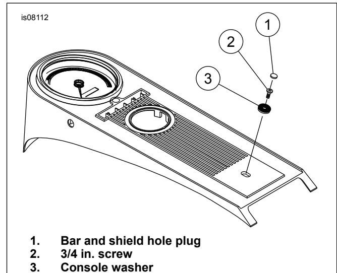
Figure 1. Installation on FLHR Instrument Panel
