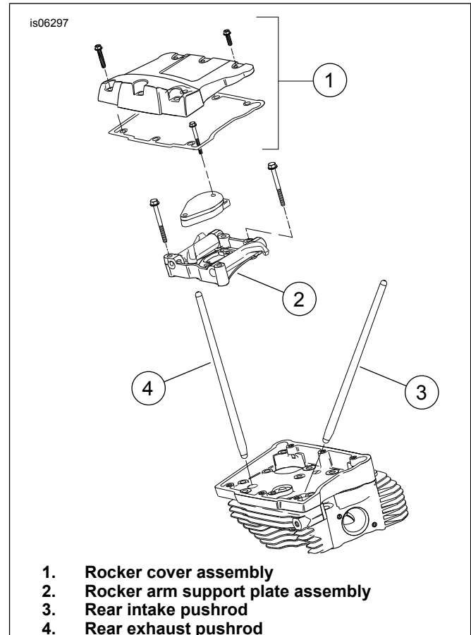
Figure 1. Push Rods
