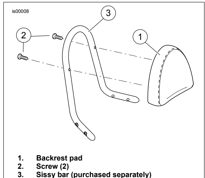
Figure 2. Generic Backrest Pad Assembly
