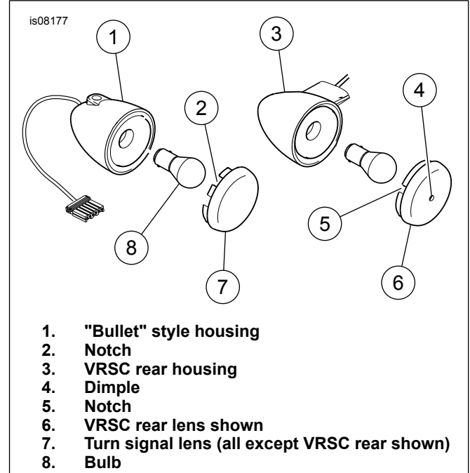
Figure 1. "Bullet" and VRSC Turn Signal Lenses
