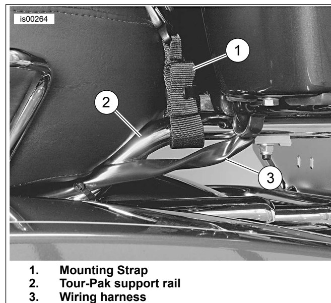
Figure 5. Avoid Pinching Wiring Harnesses
