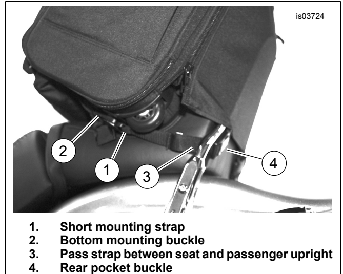
Figure 9. Strap Configuration 4
