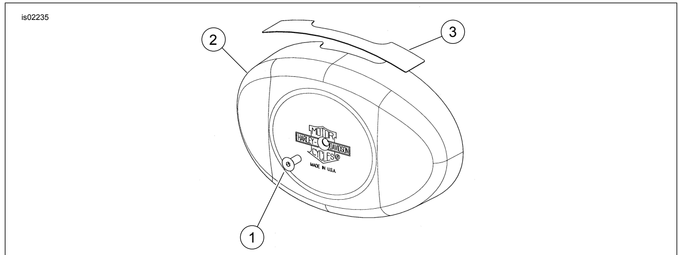
Figure 1. Service Parts: Nostalgic Twin Cam 88 Air Cleaner Cover
