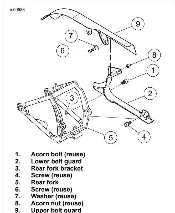
Figure 2. Stock Lower Belt Guard
