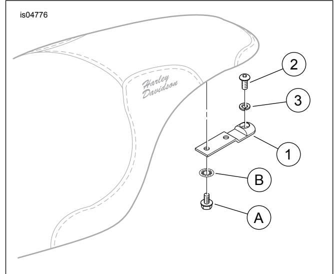
Figure 1. Service Parts, Billet Chrome Seat Bracket Kit
