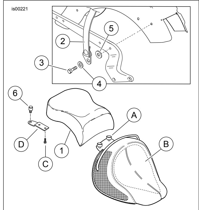
Figure 1. Service Parts: Touring Pillion Kit
