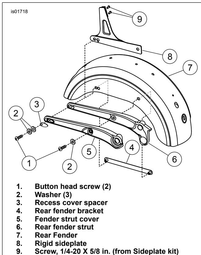
Figure 3. Sideplate Installation (Right Side Shown)
