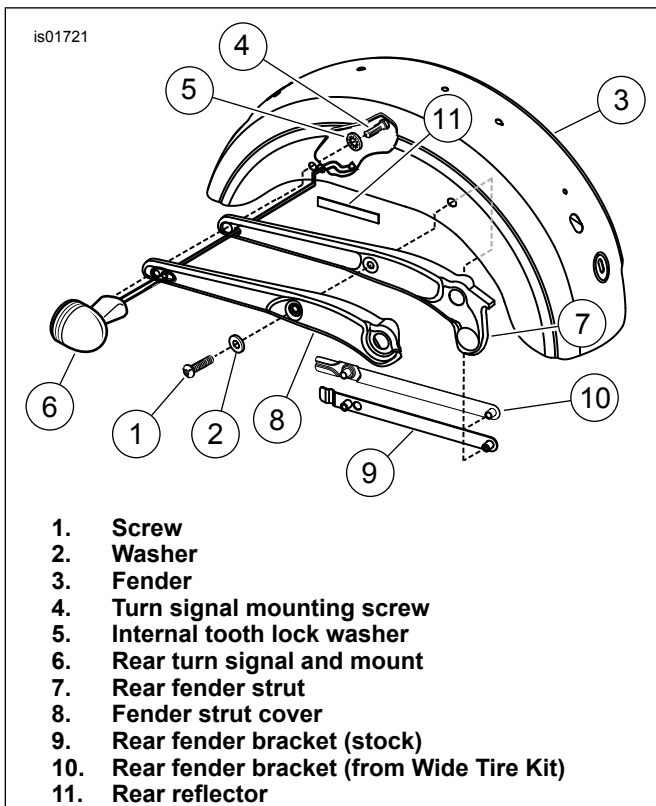
Figure 2. Remove Turn Signals and Rear Fender Bracket
