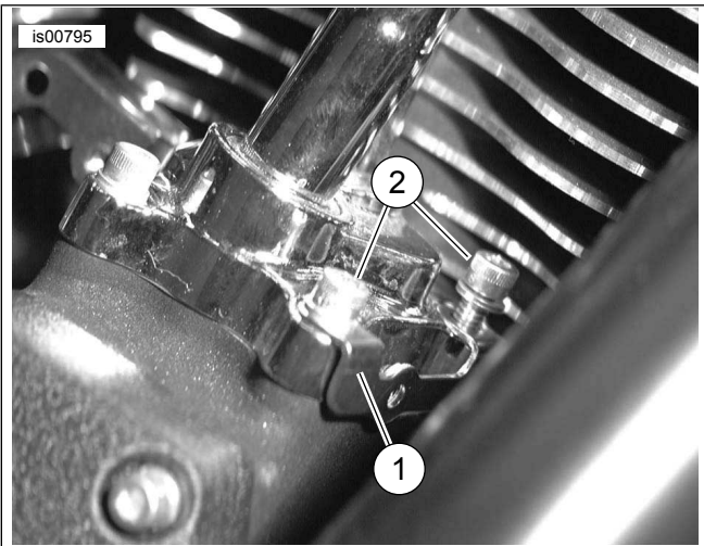
Figure 2. Front Lifter Cover Bracket Installed
