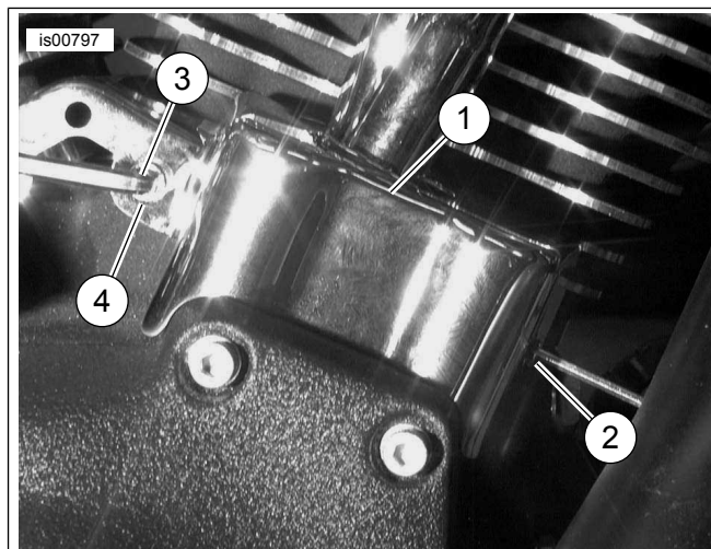
Figure 3. Center Lifter Cover Bracket Installation
