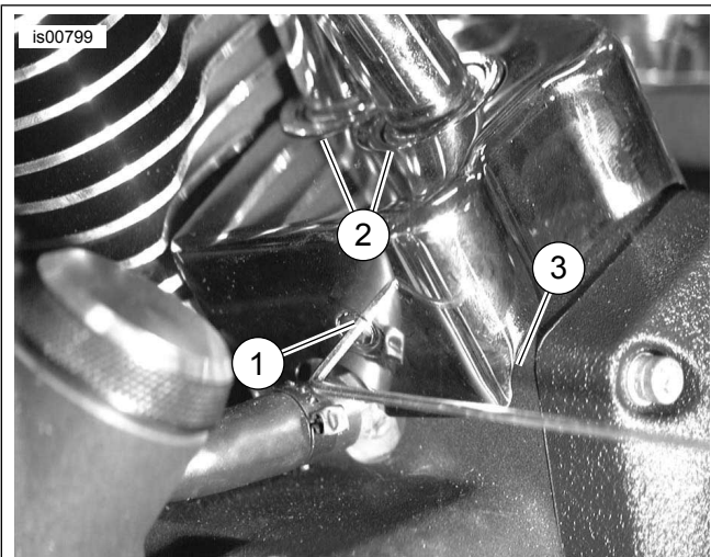
Figure 5. Cover in Correct Position
