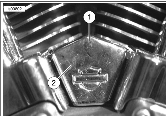
Figure 6. Lifter Cover Adjustment and Center Lifter Cover Screw Location
