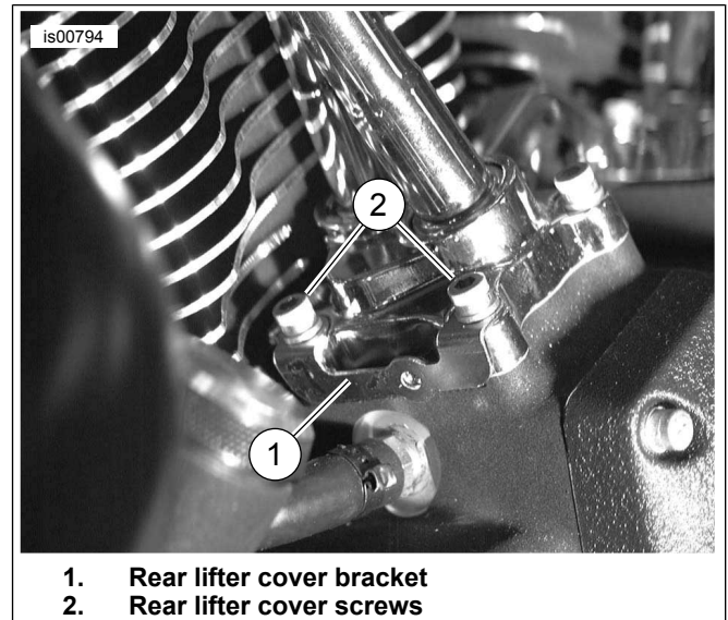
Figure 1. Rear Lifter Cover Bracket Installed
