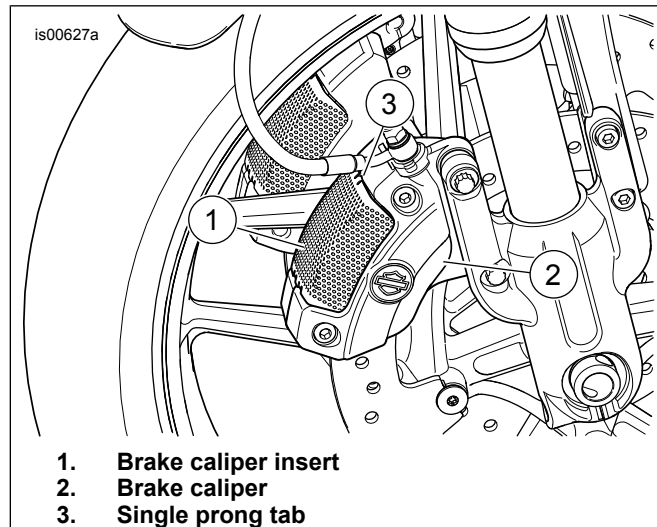
Figure 1. Front Brake Caliper (VRSCR Model Shown)
