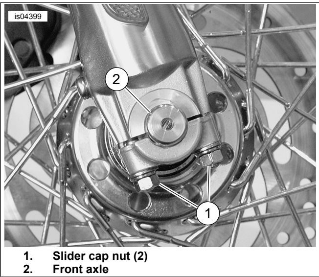
Figure 2. Front Wheel Mounting (Right side Shown)
