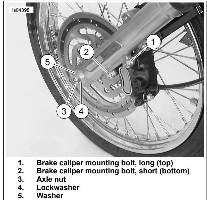
Figure 1. Caliper Mounting Bolts (Left Side Shown)
