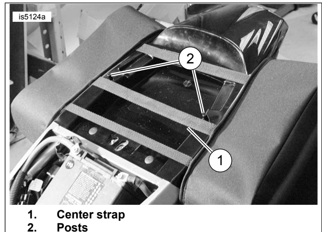
Figure 2. Saddlebag Center Straps
