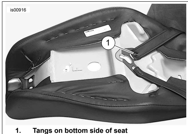
Figure 4. Underside of Seat Showing Grab Strap Installed
