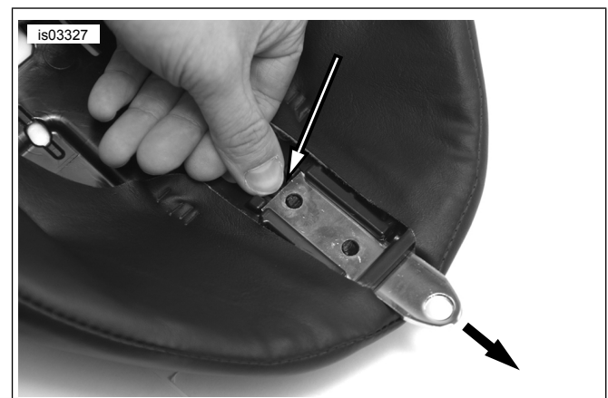
Figure 1. Seat Bracket Removal (Snap-In Bracket Shown)
