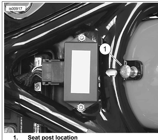
Figure 5. Seat Post
