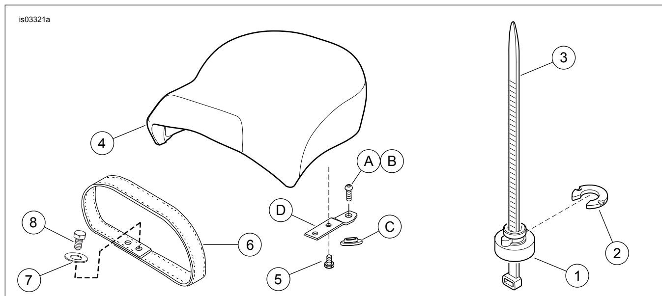
Figure 6. Service Parts: XL Passenger Pillion Kit
