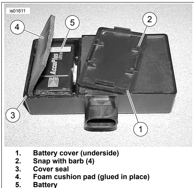
Figure 2. Remove and Replace Battery and Seal (Smart Siren)
