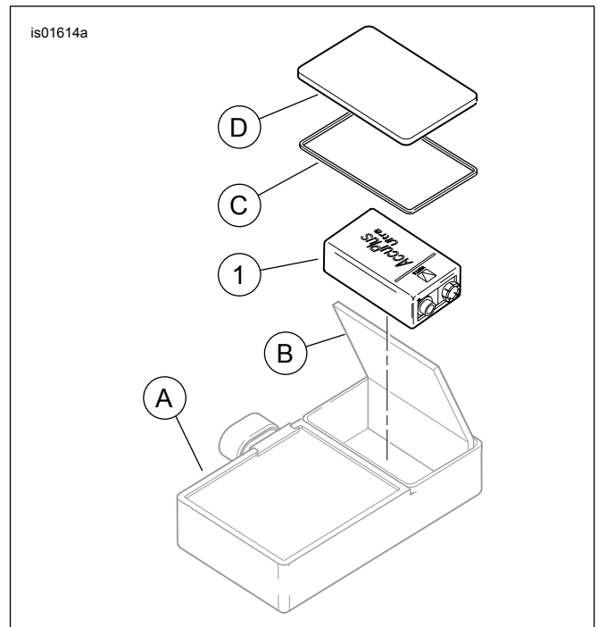
Figure 7. Service Parts, Kit 69309-10
