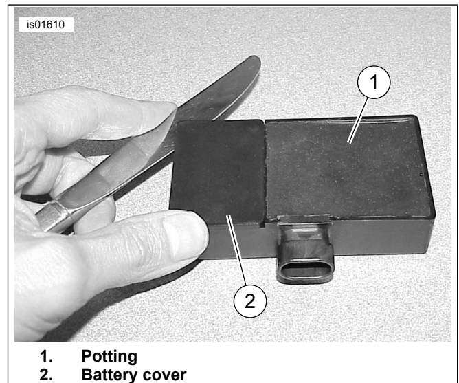
Figure 1. Insert Blade Between Case and Cover (Smart Siren)
