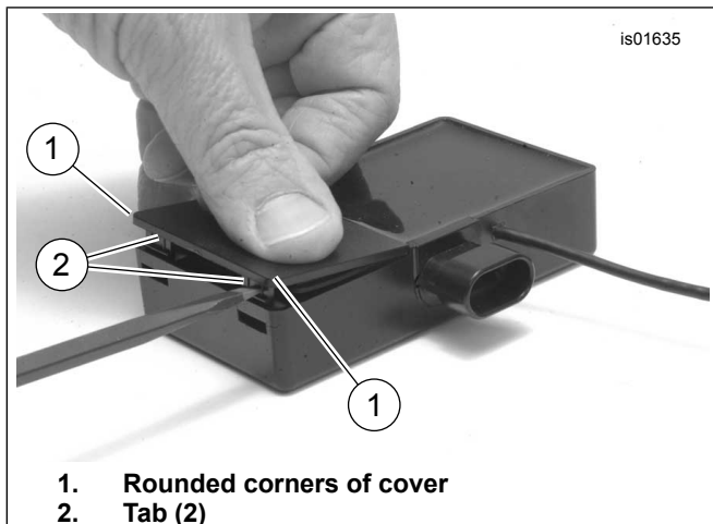
Figure 6. Snap Tabs Into Slots (Smart Siren II)
