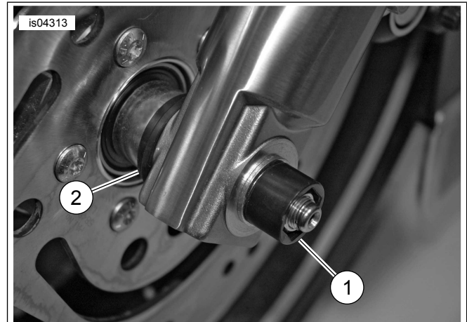
Figure 1. Install Axle Nut Cap and Axle Insert
