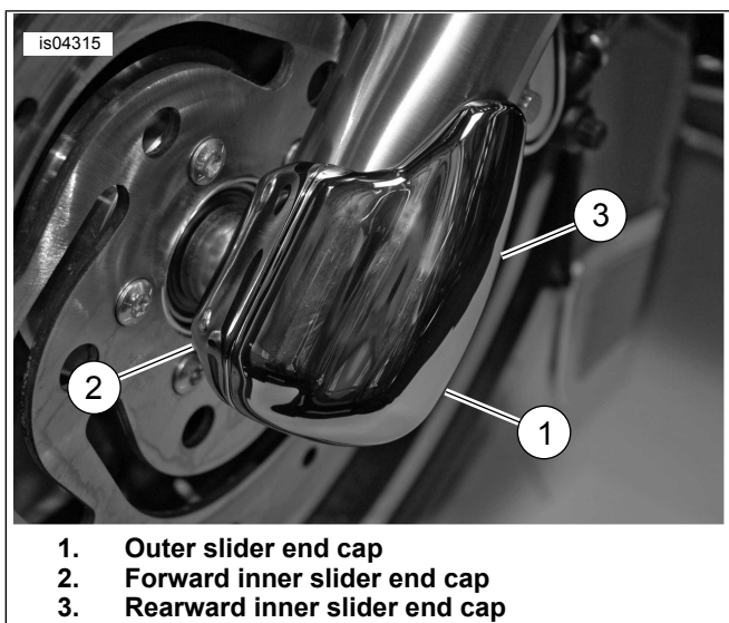
Figure 3. Install Slider End Caps (Left Side Shown)
