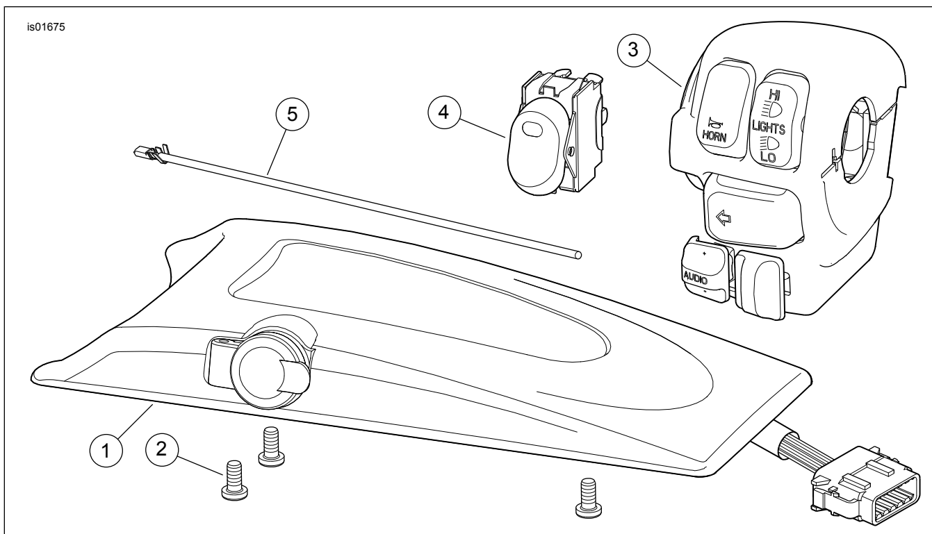
Figure 1. Service Parts, Kit 77173-06
