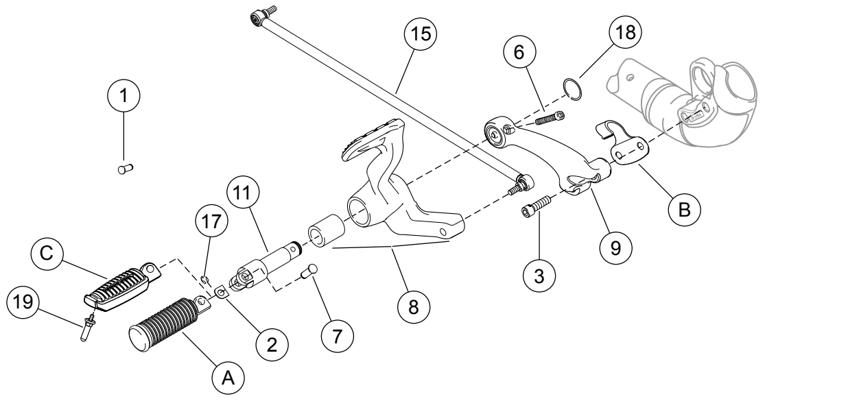
Figure 7. Service Parts: Forward Control, Right (Brake) Side
