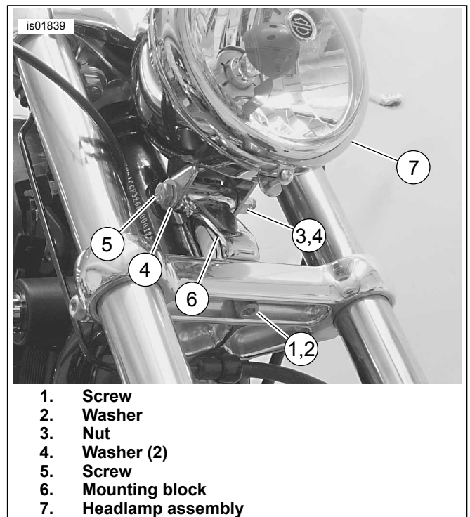
Figure 6. Sportster Headlamp Assembly with Mount
