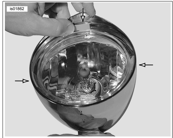
Figure 15. Place Two-Sided Tape on Chrome Trim Ring
