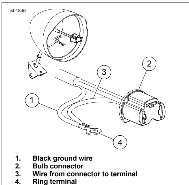
Figure 9. Clip Black Ground Wire
