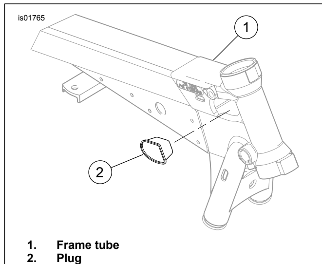
Figure 4. Dyna Top Frame Tube (2005-Earlier)
