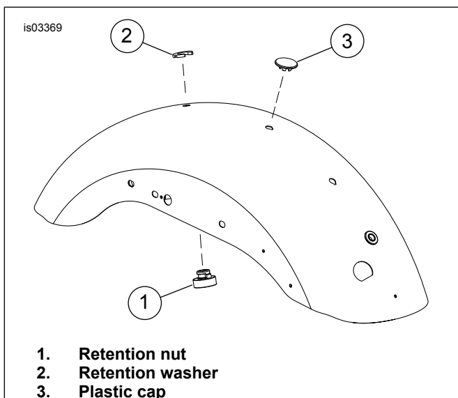
Figure 3. Retention Nut and Plastic Cap (2-Up Seats)
