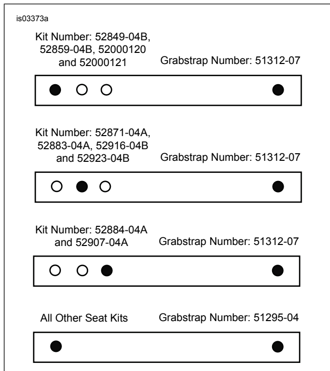
Figure 6. Grabstrap Installation
