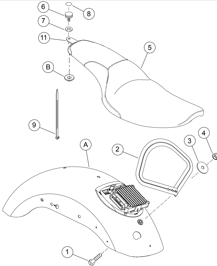
Figure 7. Service Parts: XL 2-Up Custom Seat Kits
