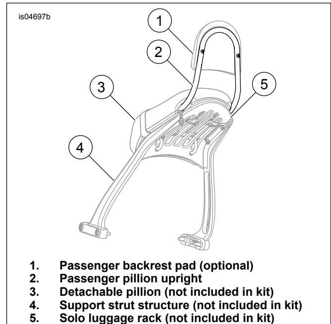
Figure 1. FXCW Passenger Pillion Upright
