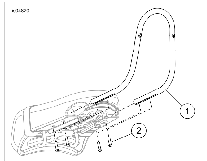
Figure 2. Service Parts: FXCW Passenger Pillion Upright Kit
