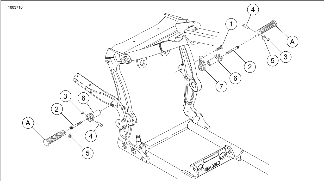
Figure 1. Service Parts, Passenger Footpeg Support Kit
