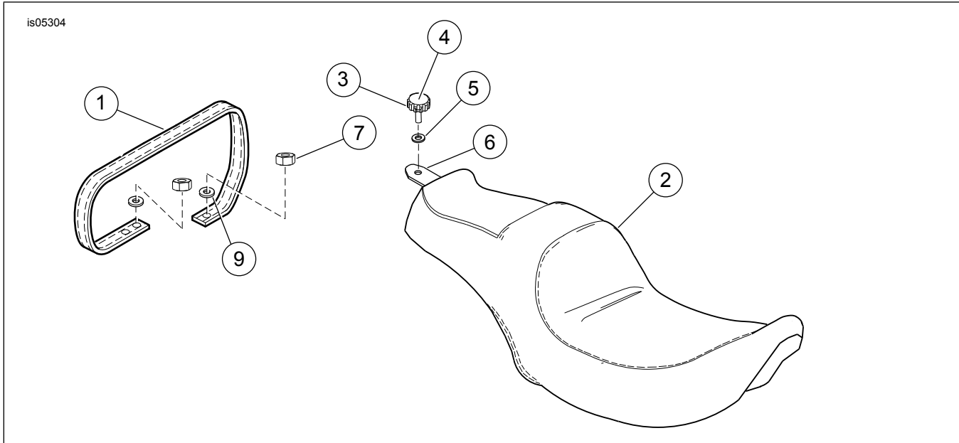
Figure 4. Service Parts: Two-Up Seat Kits for Touring Models
