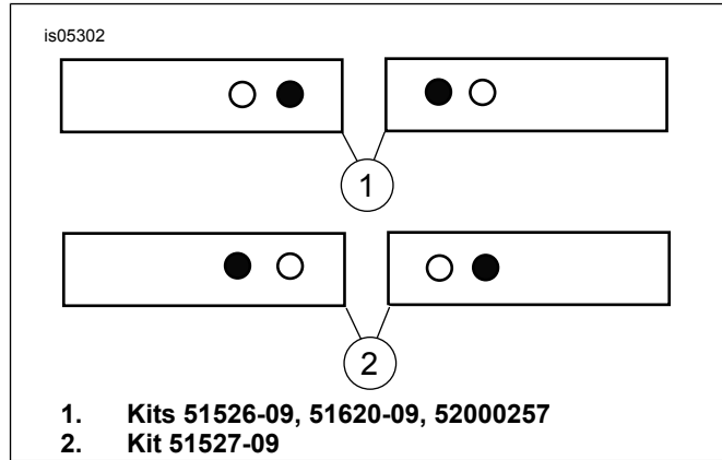
Figure 3. Grab Strap Installation
