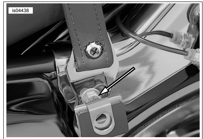
Figure 2. Passenger Grab Strap Removal (2008 Shown)
