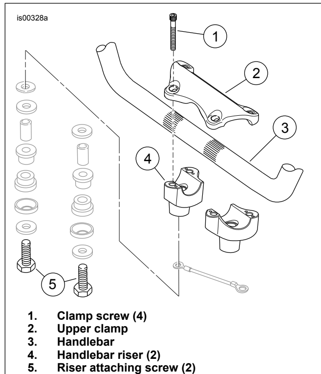
Figure 1. Handlebar Clamp and Risers
