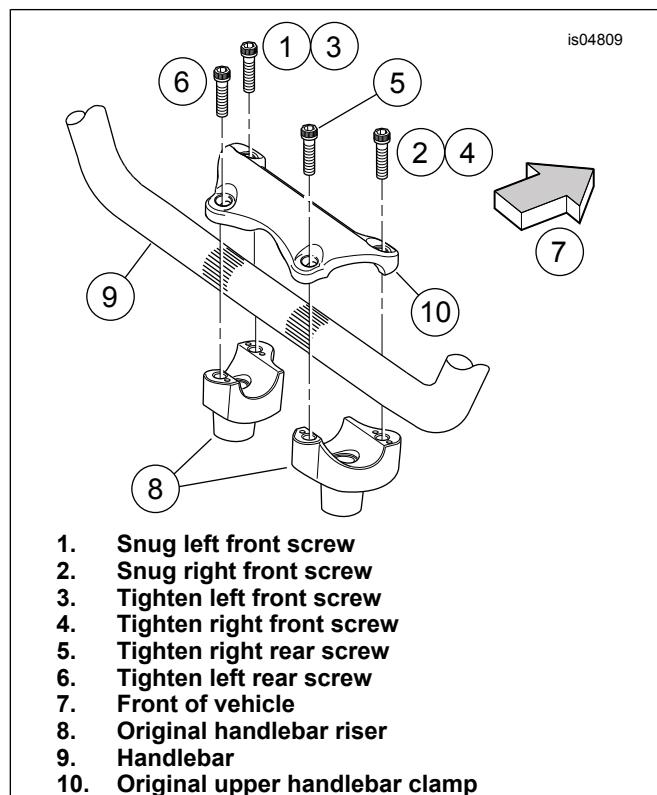
Figure 3. Handlebar Clamp Screw Tightening Sequence
