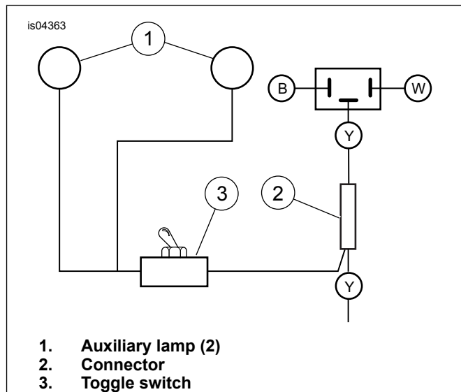
Figure 3. Wiring Diagram
