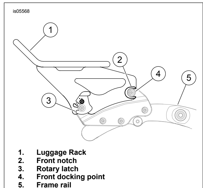
Figure 1. Luggage Rack
